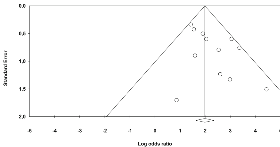
Fig. 3 Funnel plot of the natural logarithm-transformed odds ratio estimates, by the corresponding standard error. Circles, studies in the meta-analysis
