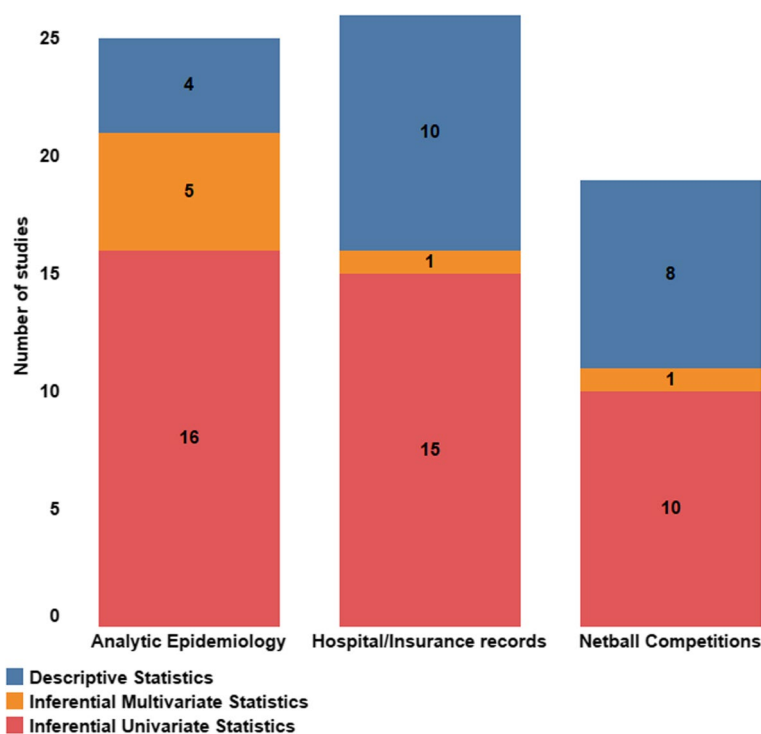
Fig. 2 Frequency of Netball injury studies by study design and data analysis methods
